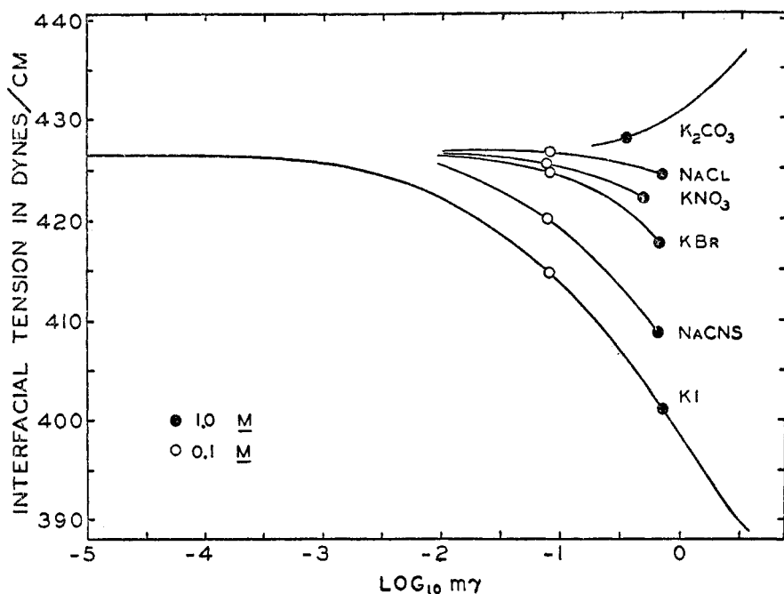
FIG. 7. Maximum interfacial tension of mercury in contact with aqueous solutions of the salts named. T = 18^\circ\text{C} . Data by Gouy (36). The slope measures the amount of salt adsorbed (equations 19 and 21). (Additional points not shown were used in the construction of the figure.)
