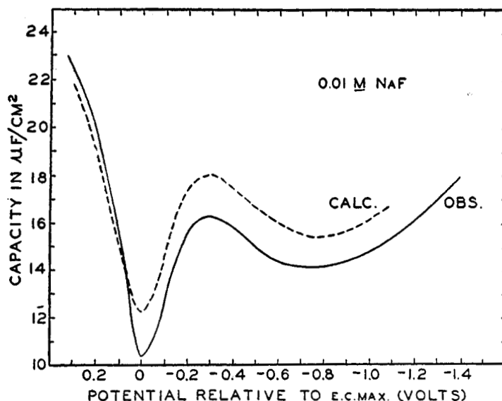
FIG. 13. Calculated and observed differential capacity of mercury in contact with 0.01 M sodium fluoride. T = 25^{\circ}\text{C} . Experimental data obtained with 1.0 M sodium fluoride enter into these calculations.
